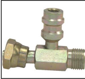
Female O-Ring to Male Insert O-Ring w/R134a Service Port
