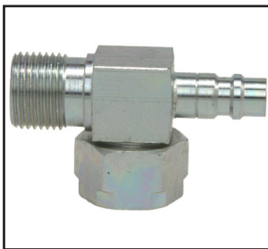
90° Tube-O to Male Insert O-Ring w/R134a Service Port
