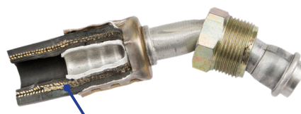
Layers Lose Elasticity & Leak at Crimp Connections
