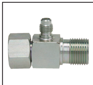
Female O-Ring to Male Insert O-Ring w/R12 Service Port
