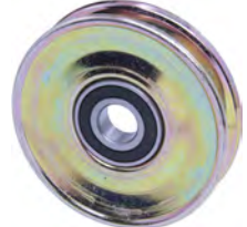
934121 Idler / Tensioner Pulley V-Belt Groove: 1 Pulley Dia.: 3-1/2 Belt Width: 1/2 FORD (96)
